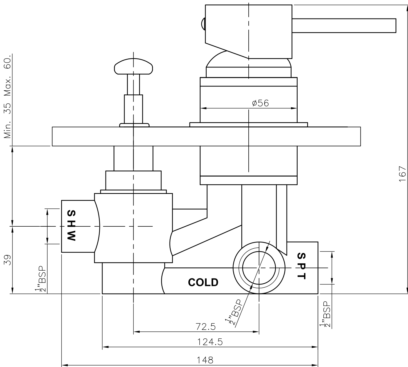
RUBBIC - F190019 - HIGH FLOW SINGLE LEVER CONCEALED MIXER FOR BATH & SHOWER SYSTEM
