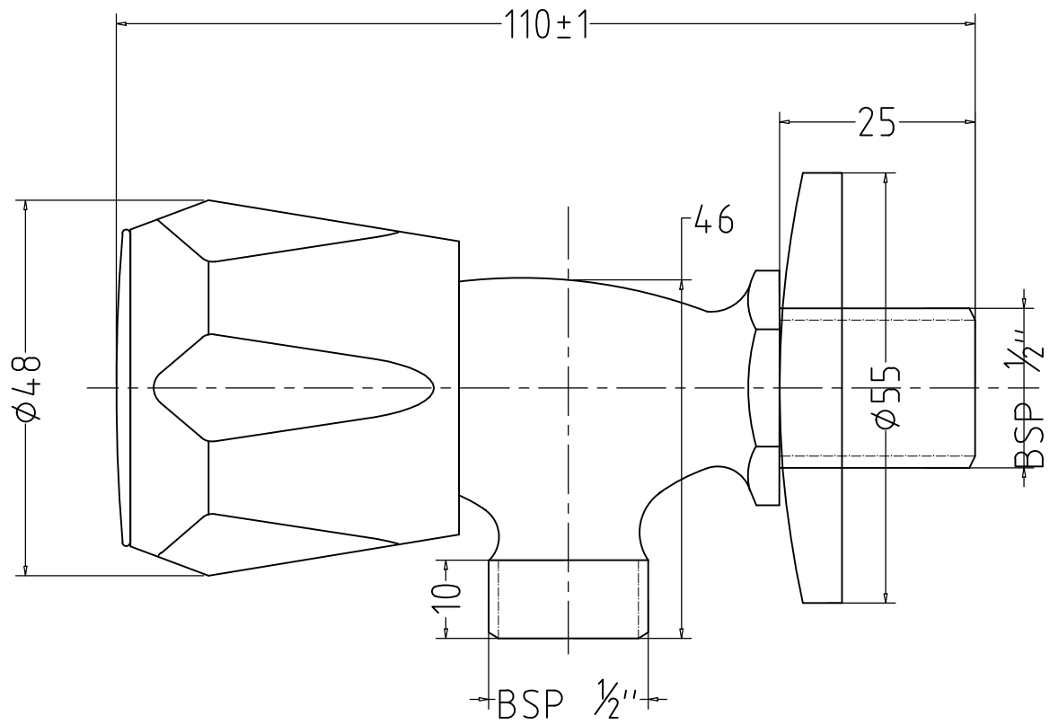
CLASSIK F200005 ANGULAR STOP COCK (WITH WALL FLANGE)
