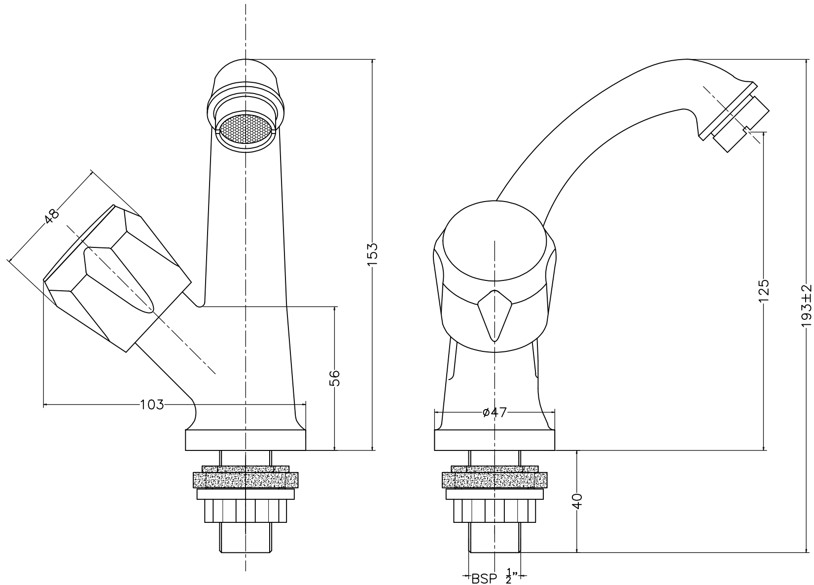
CLASSIK:F200012 SWAN NECK TAP WITH LEFT HAND OPERATING KNOB
