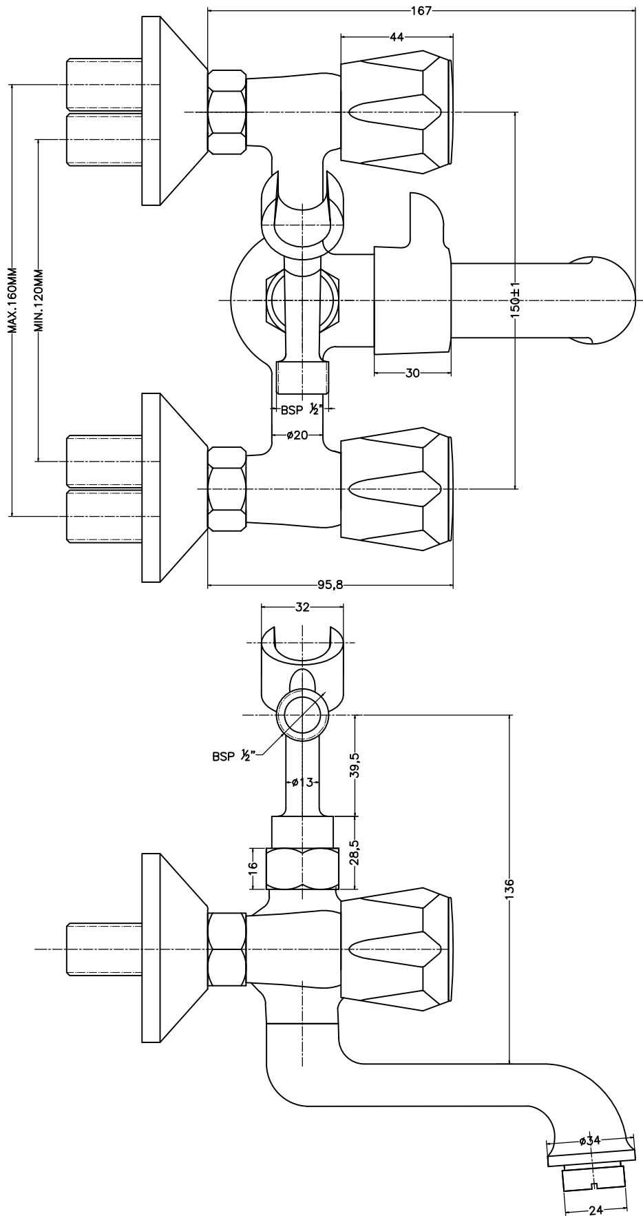
CLASSIK-F200018-WALL MIXER WITH HAND SHOWER ARRANGEMENT ONLY WITH CRUTCH
