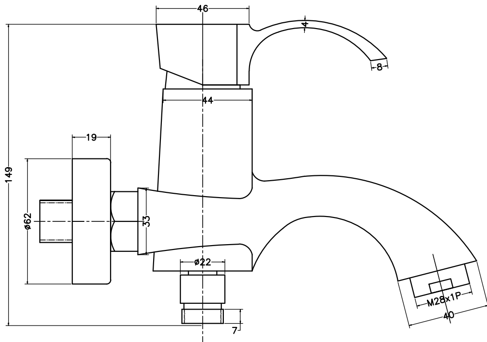
CORNICE- F230011 SINGLE LEVER BATH & SHOWER MIXER EXPOSED
