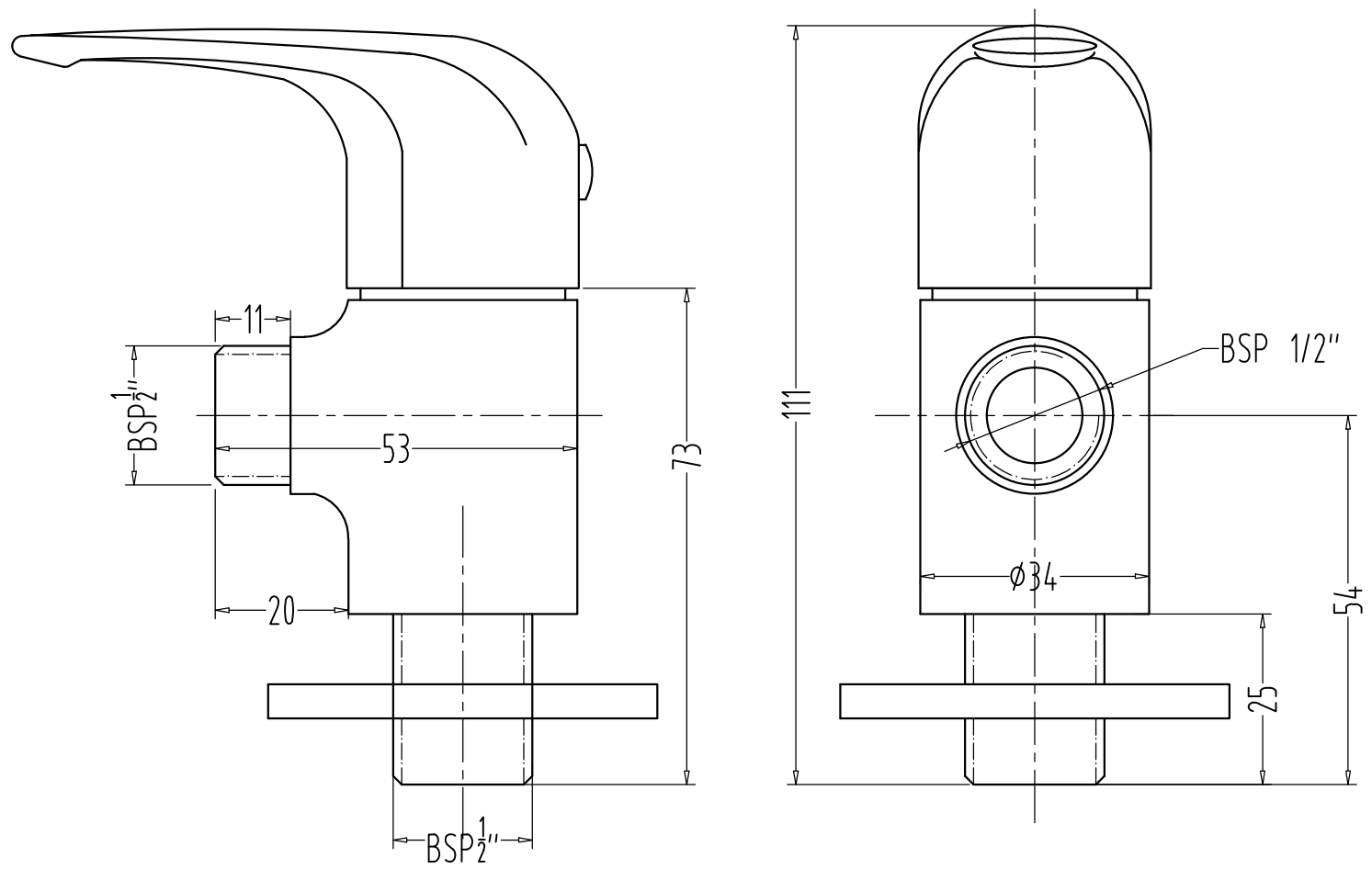
ESSENCE F130003 ANGULAR STOP COCK
