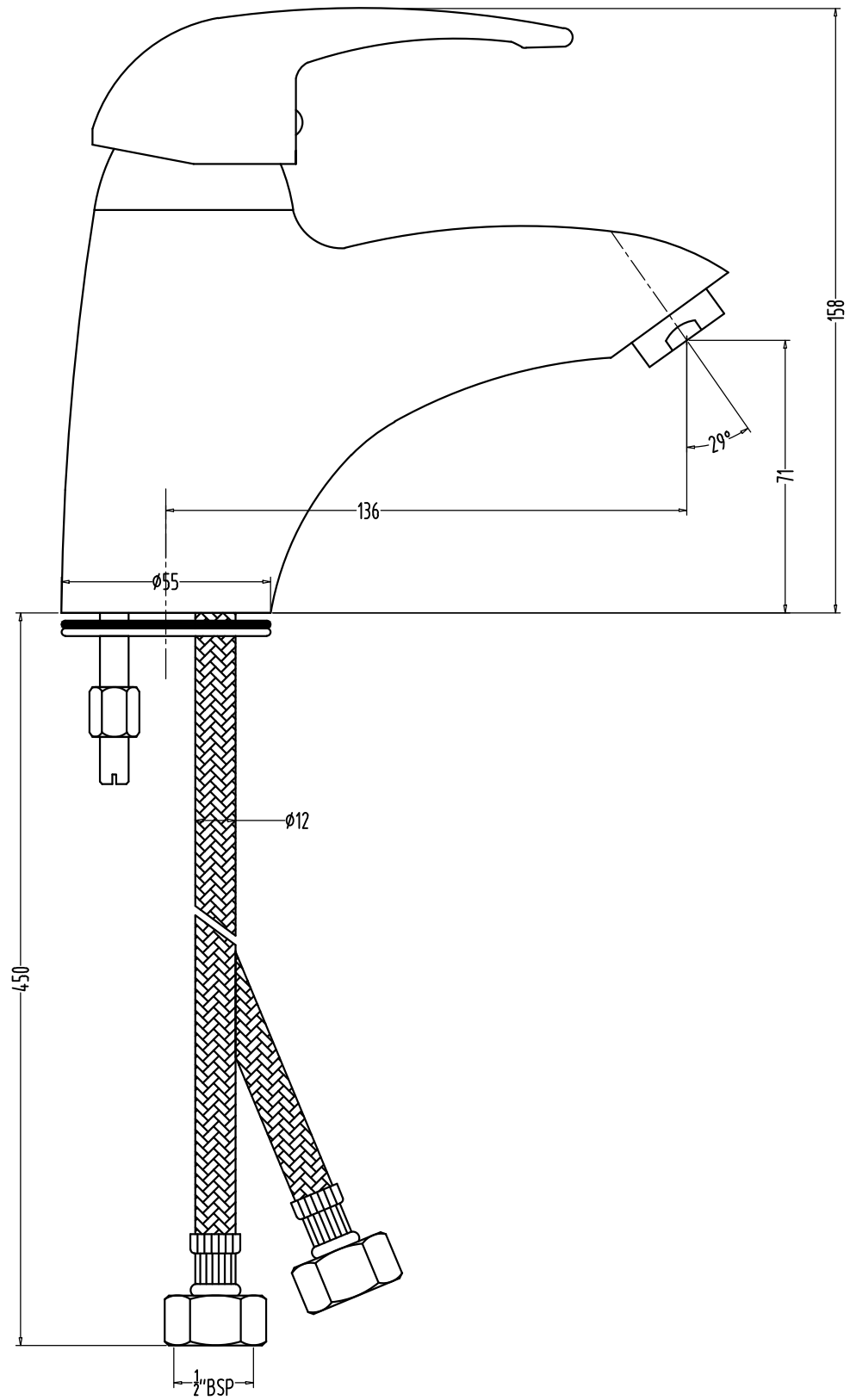
ESSENCE F130010 SINGLE LEVER BASIN MIXER W/O POPUP WASTE
