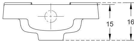
FRONT ELEVATION
