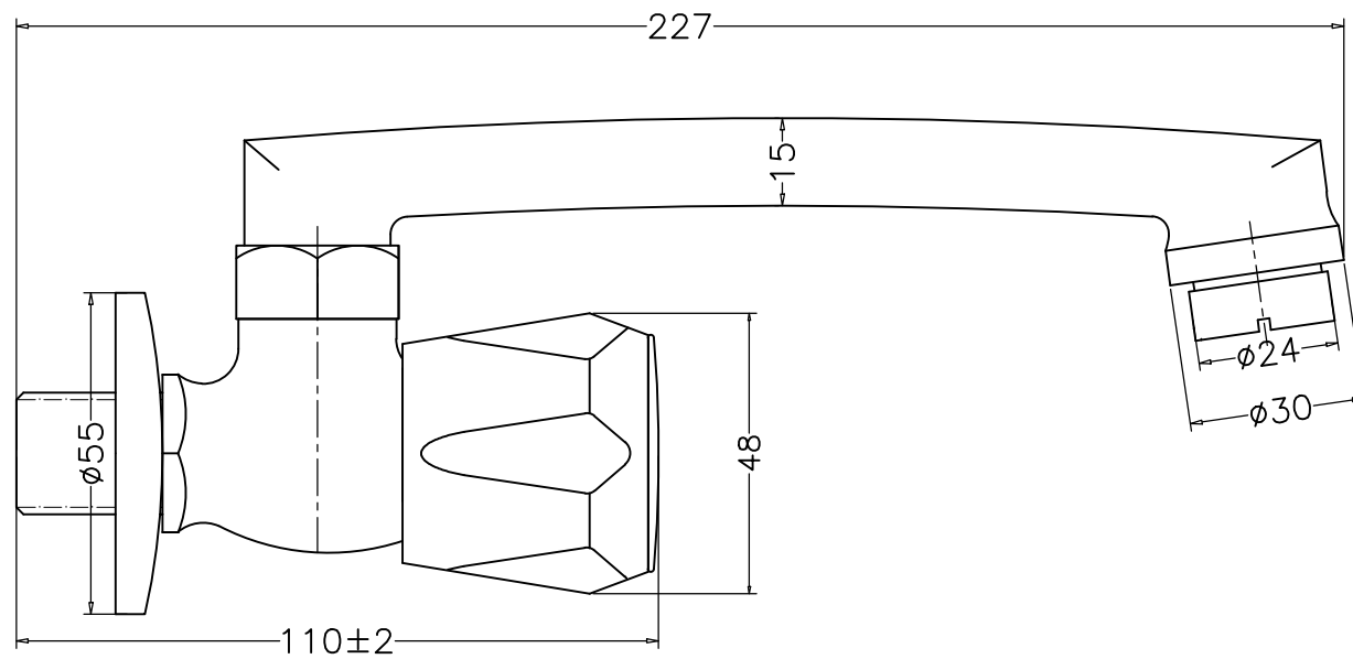
CLASSIK—F200024—SINK COCK WITH SWIVEL CASTED SPOUT
