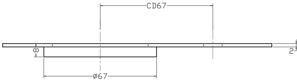
WALL FLANGE
