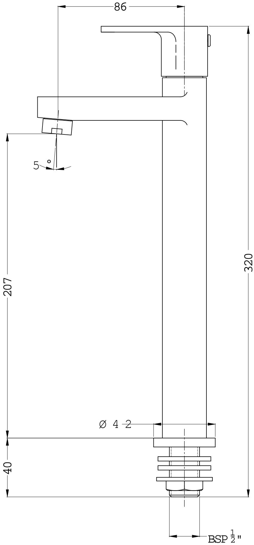
CORA-F440002 PILLAR COCK(TALL)
