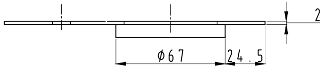
WALL FLANGE WITH 'O'RING
