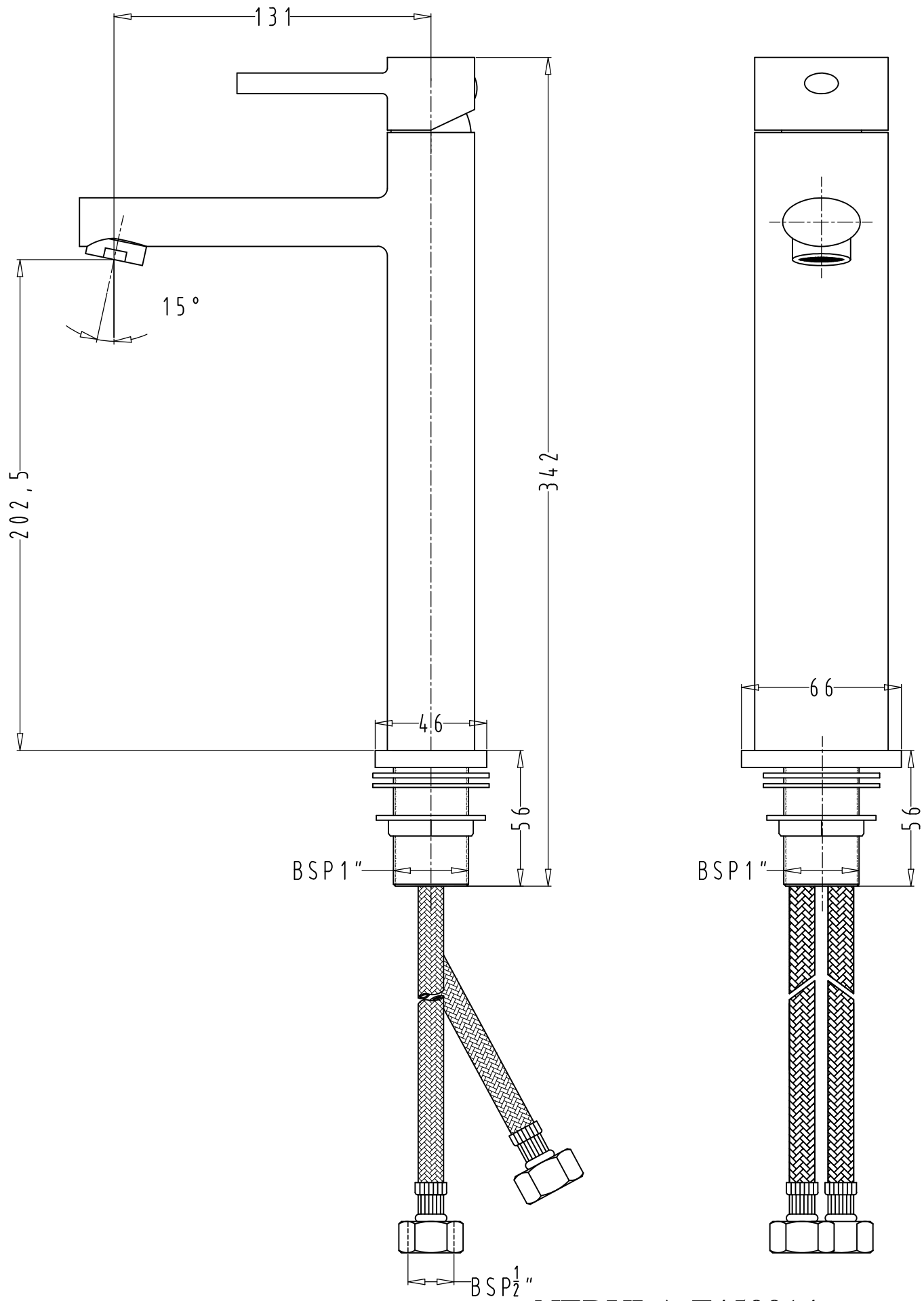
NEBULA-F450014 SL BASIN MIXER (TALL)
