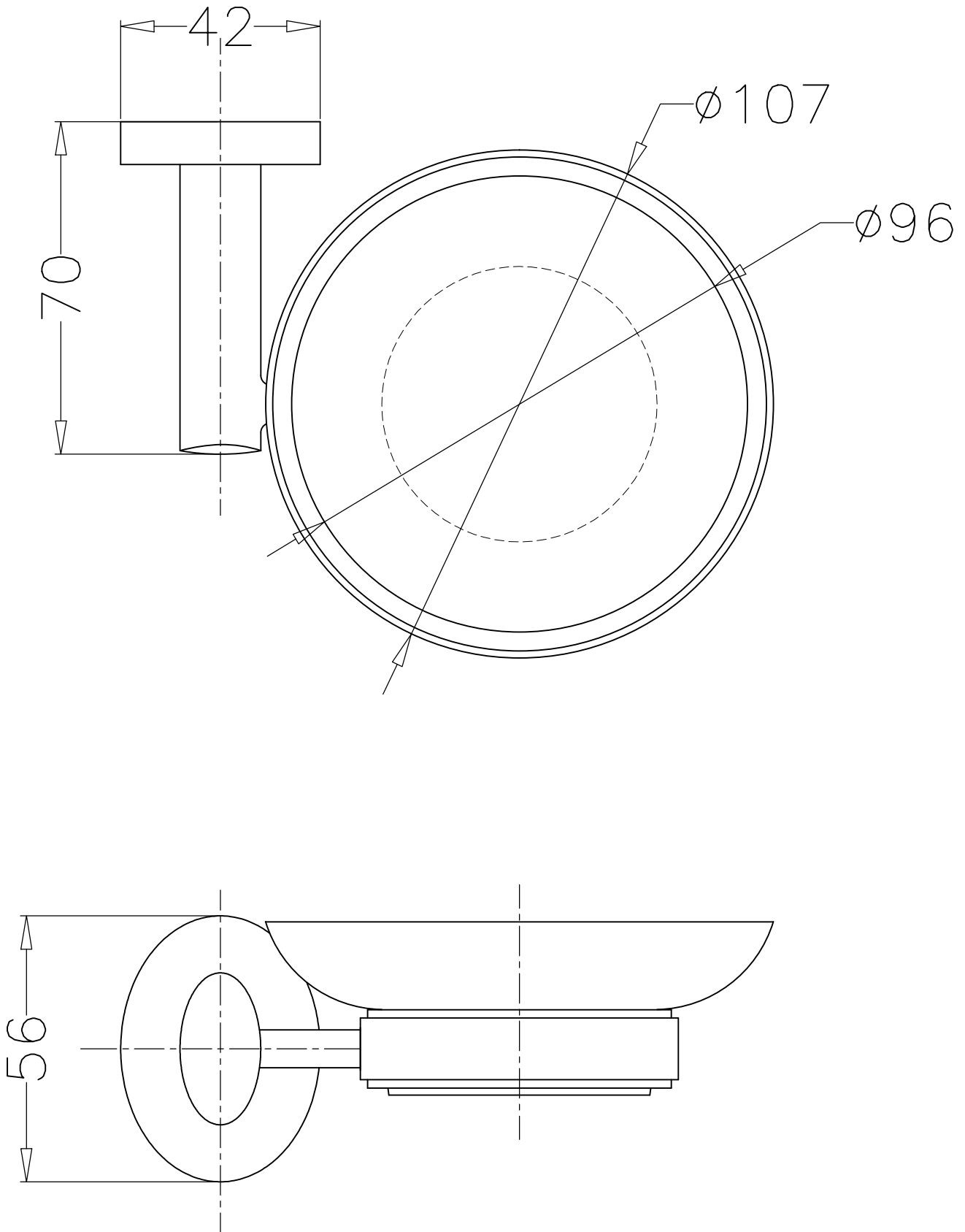
NEBULA-F450025CP TUMBLER HOLDER
