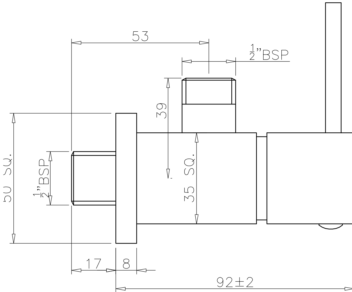
RUBBIC-F190003- ANGULAR STOP COCK SQ. WITH WALL FLANGE
