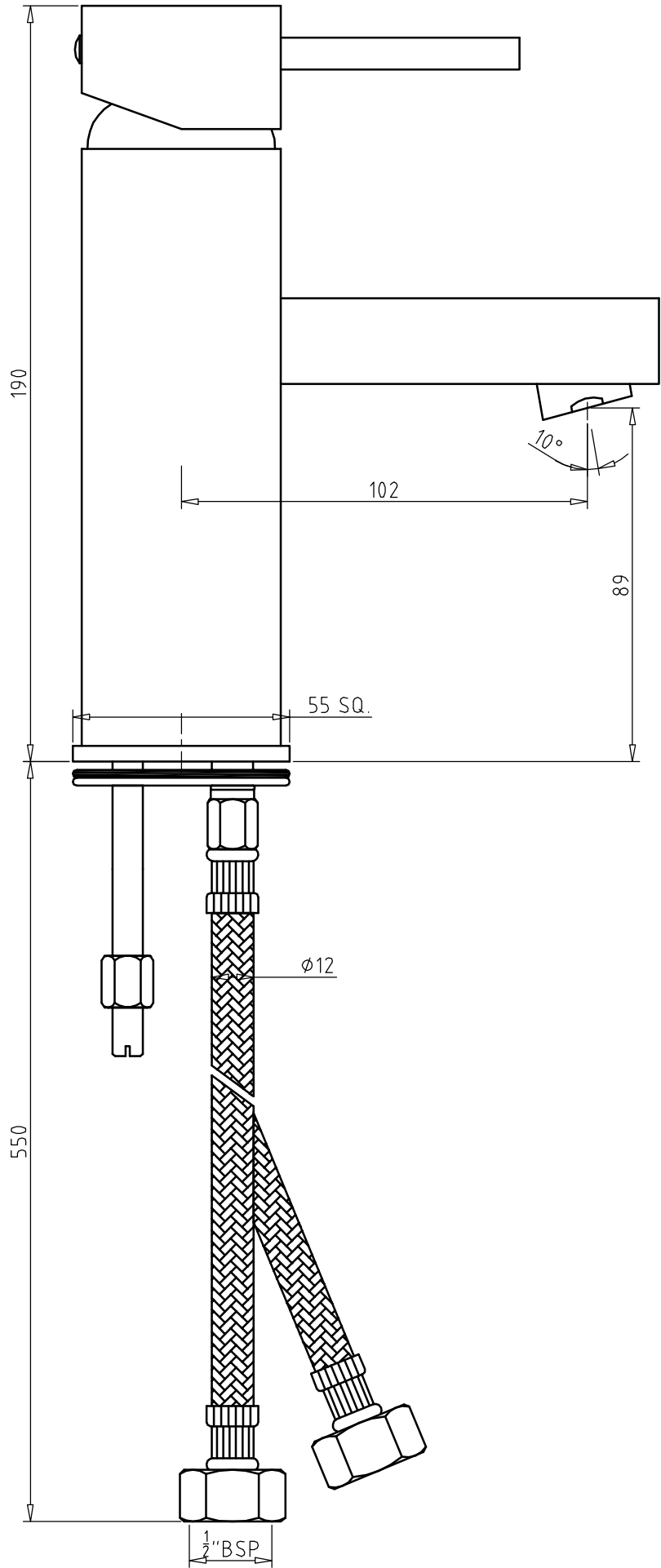
RUBBIC- F190009 -SINGLE LEVER BASIN MIXER WITHOUT POPUP WASTE SYSTEM SQUARE WITH 550 MM STAINLESS STEEL FLEXIBLE HOSE
