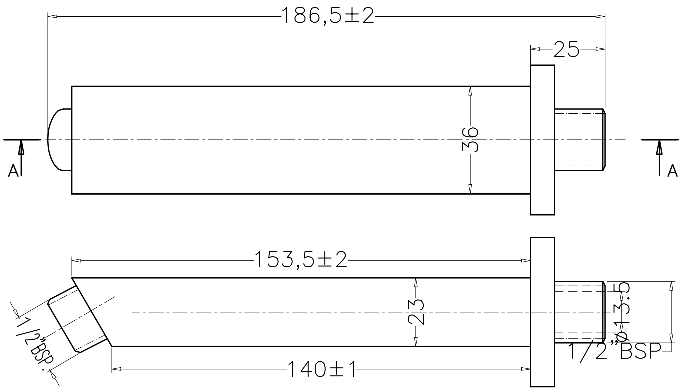
RUBBIC: F190018 Shower Arm
