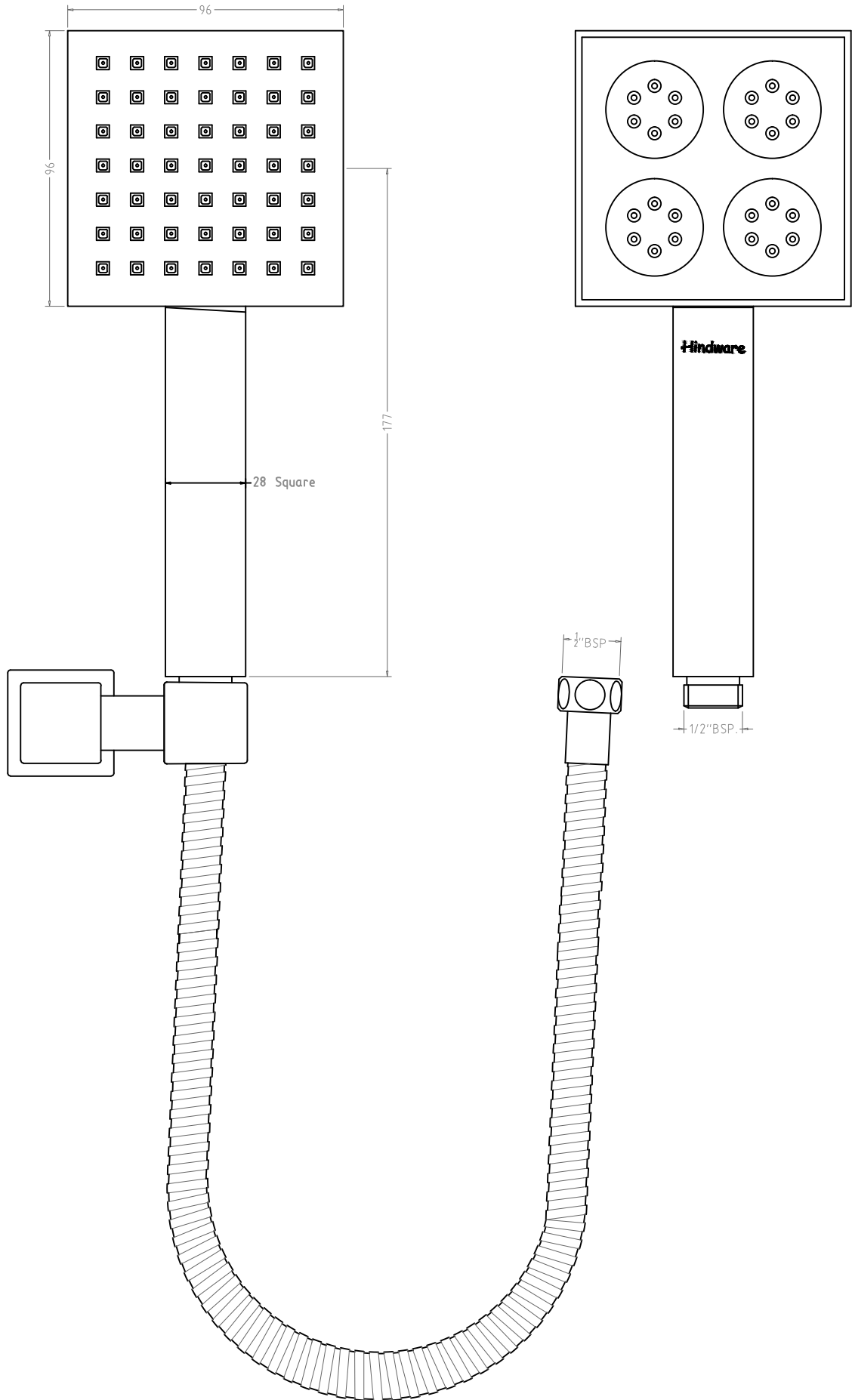
SHOWERS-F 160020-2 WAY SQUARE IMPORTED HAND SHOWER WITH DOUBLE LOCK 150 CM BRASS PLATED FLEXIBLE HOSE & WALL HOOK.
