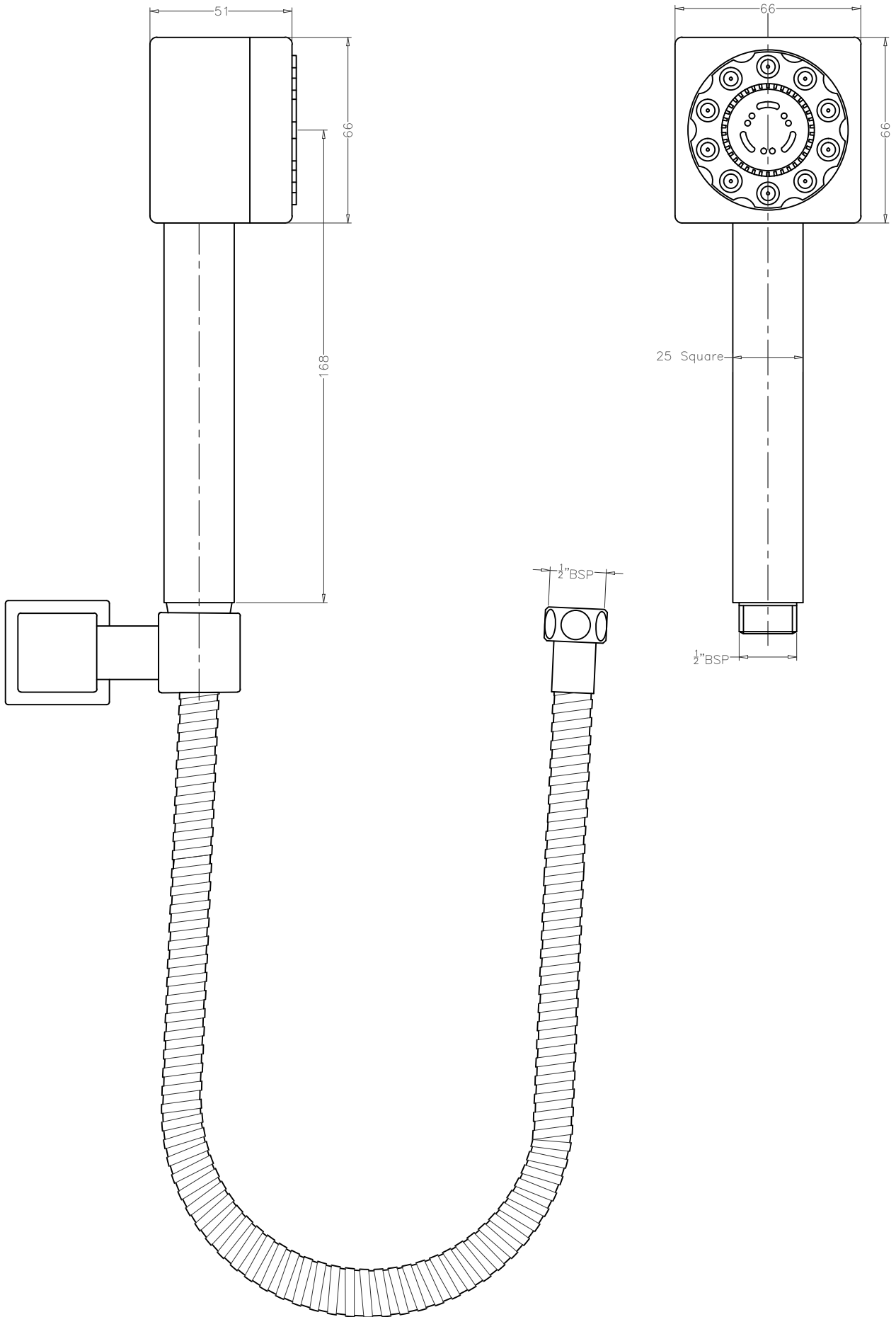
SHOWERS -F160021- THREE FLOW SQUARE IMPORTED HAND SHOWER WITH DOUBLE LOCK 150 cm BRASS PLATED FLEXIBLE HOSE & WALL HOOK. DATE-19.01.16
