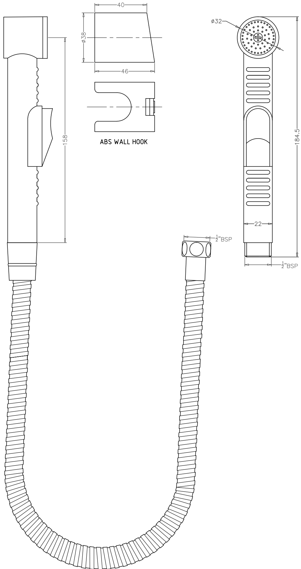
SHOWERS-F160023-HEALTH FAUCET (ABS) IMPORTED WITH 120 cm SS FLEXIBLE TUBE & ABS WALL HOOK
