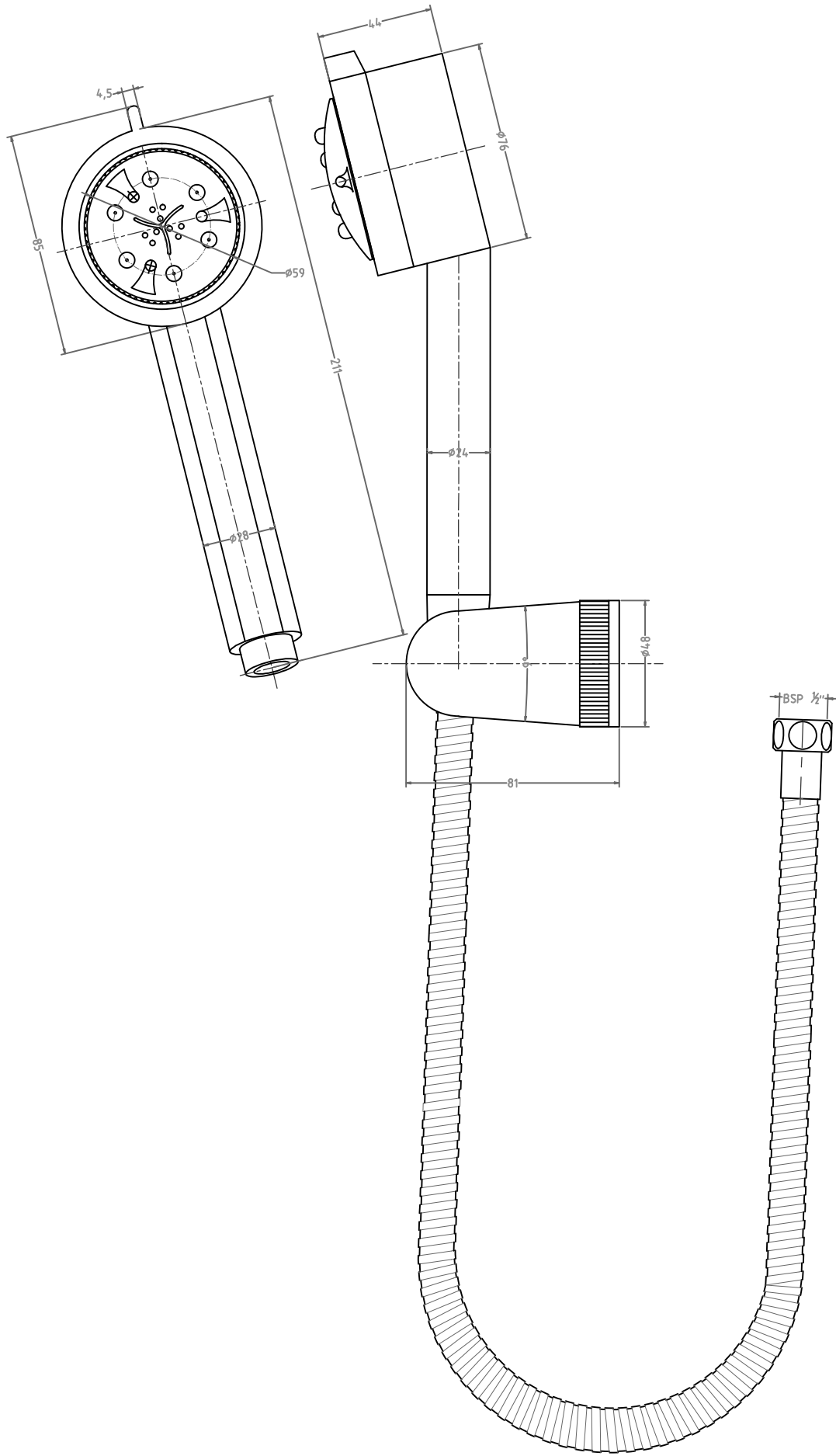
SHOWER-F160031- 5 FLOW HAND SHOWER WITH (RUBIT CLEANING SYSTEM) AND 150CM LONG PVC TUBE SWIVEL WALL HOOK WITH OPENER
