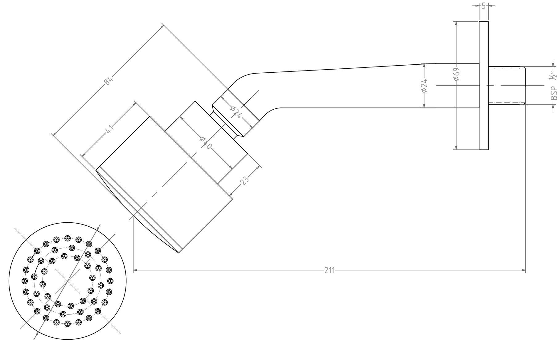
SHOWER-F160039-OVERHEAD SHOWER WITH ARM & FLANGE (PROJECT)
