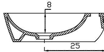
SECTIONAL VIEW
