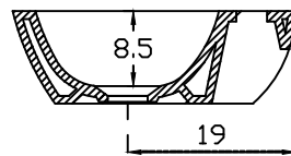
SECTIONAL VIEW
