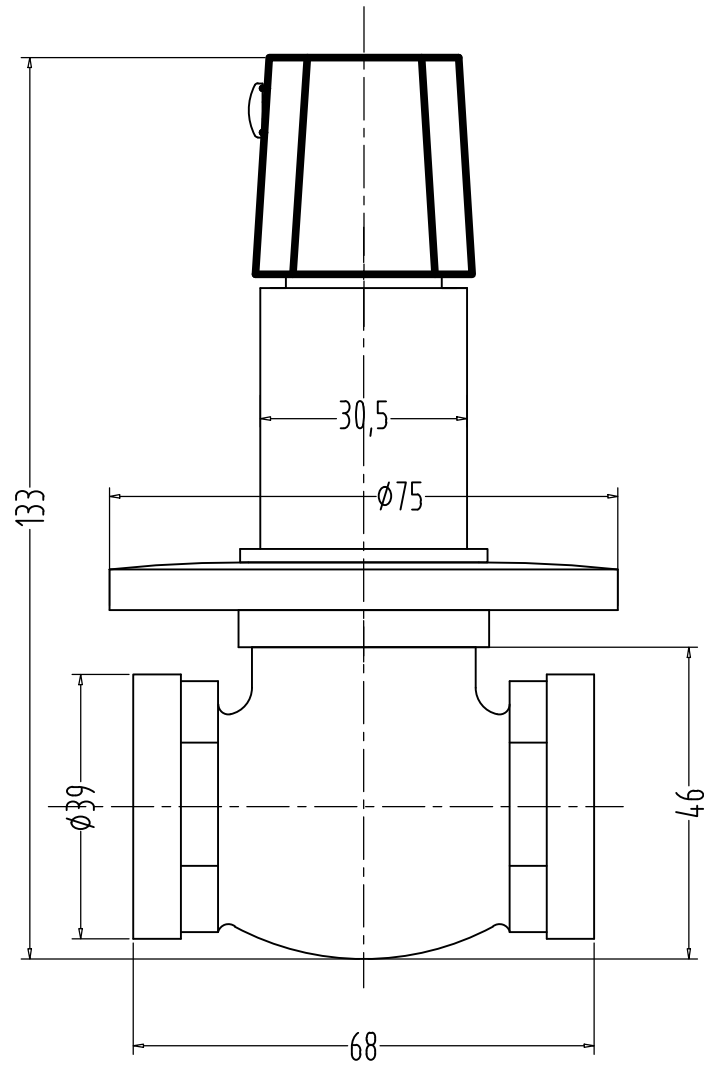
ARMADA F260006 CONCEALED STOP COCK WITH ADJ. WALL FLANGE (20MM)
