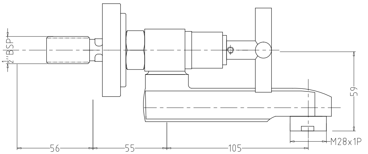
AXXIS -F120016-WALL MIXER WITHOUT HAND SHOWER ARRANGEMENT .
