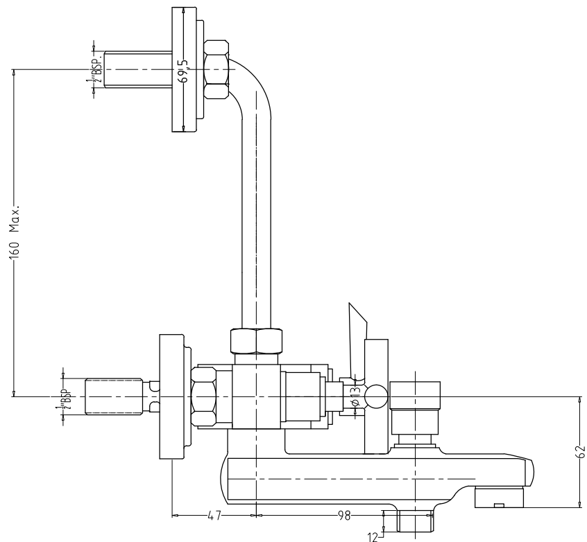
AXXIS -F120019 -WALL MIXER 3 IN 1 SYSTEM WITH PROVISION FOR BOTH HAND AND OVER HEAD SHOWER WITH 115MM. LONG BEND PIPE & WALL FLANGE.
