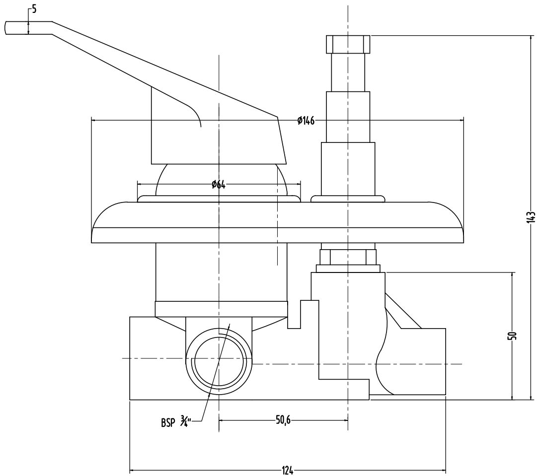
SKIPPER -F210011 SINGLE LEVER CONCEALED MIXER FOR BATH & SHOWER SYSTEM.
