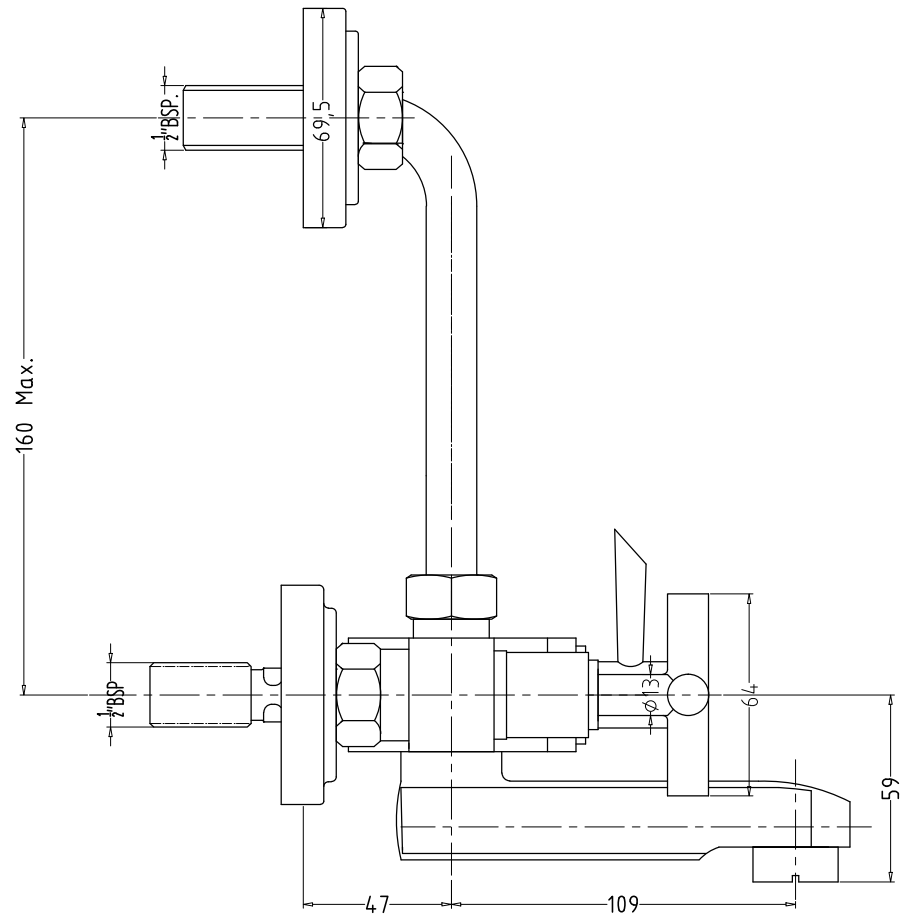
AXXIS-F120018 -WALL MIXER WITH PROVISION FOR OVER HEAD SHOWER WITH 115MM. LONG BEND PIPE & WALL FLANGE.
