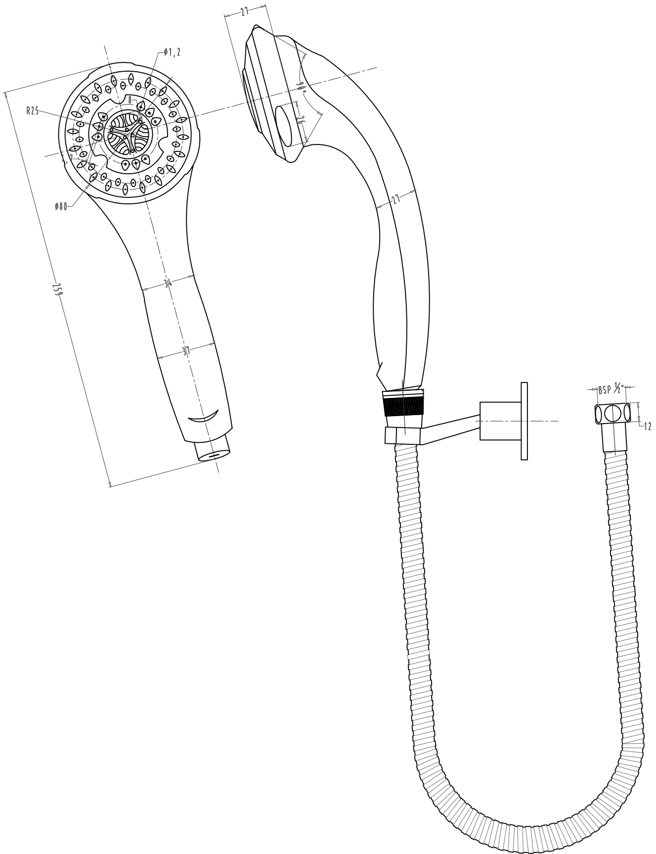
SHOWER- F160055-5 FLOW HAND SHOWER WITH 1.5MCP FLEXIBLE TUBE WITH HOOK
