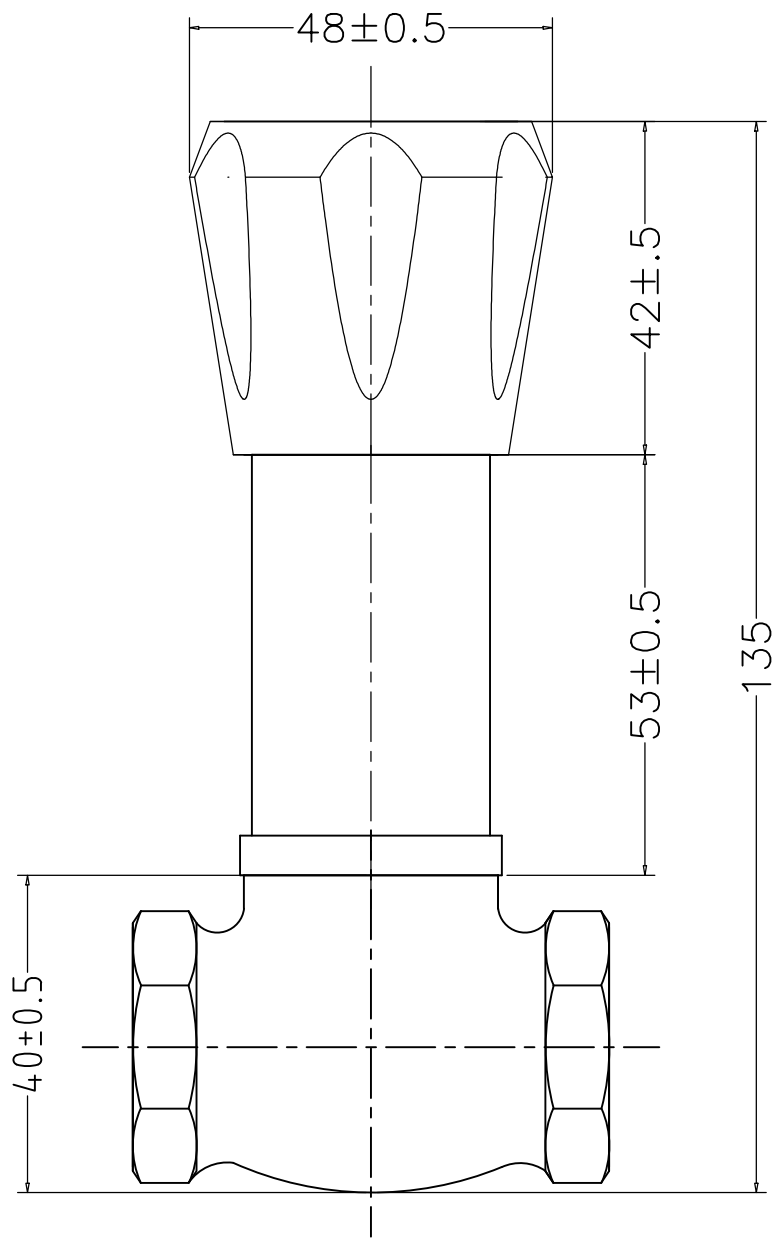
CLASSIK F200008 CONCEALED STOP COCK 20MM
