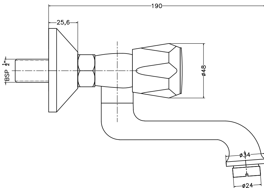
CLASSIK-F200019 WALL MIXER WITHOUT HAND SHOWER ARRANGEMENT
