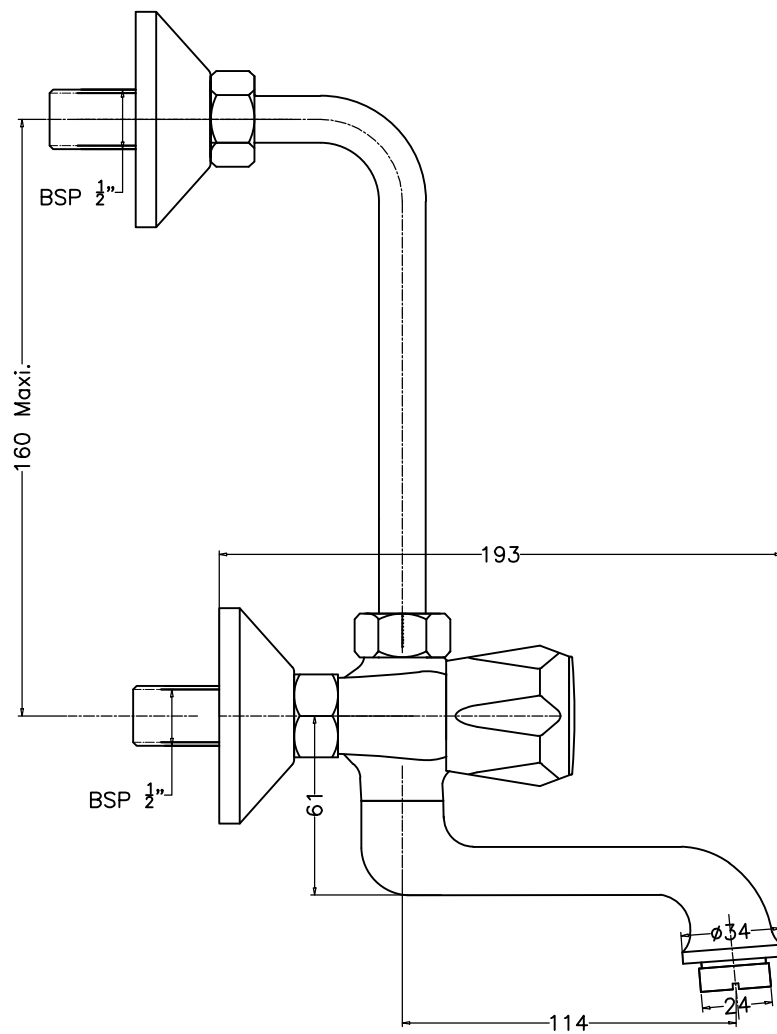
CLASSIK- F200020-WALL MIXER WITH PROVISION FOR OVER HEAD SHOWER WITH 115MM LONG BEND PIPE & WALL FLANGE
