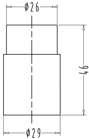
SLEEVE
