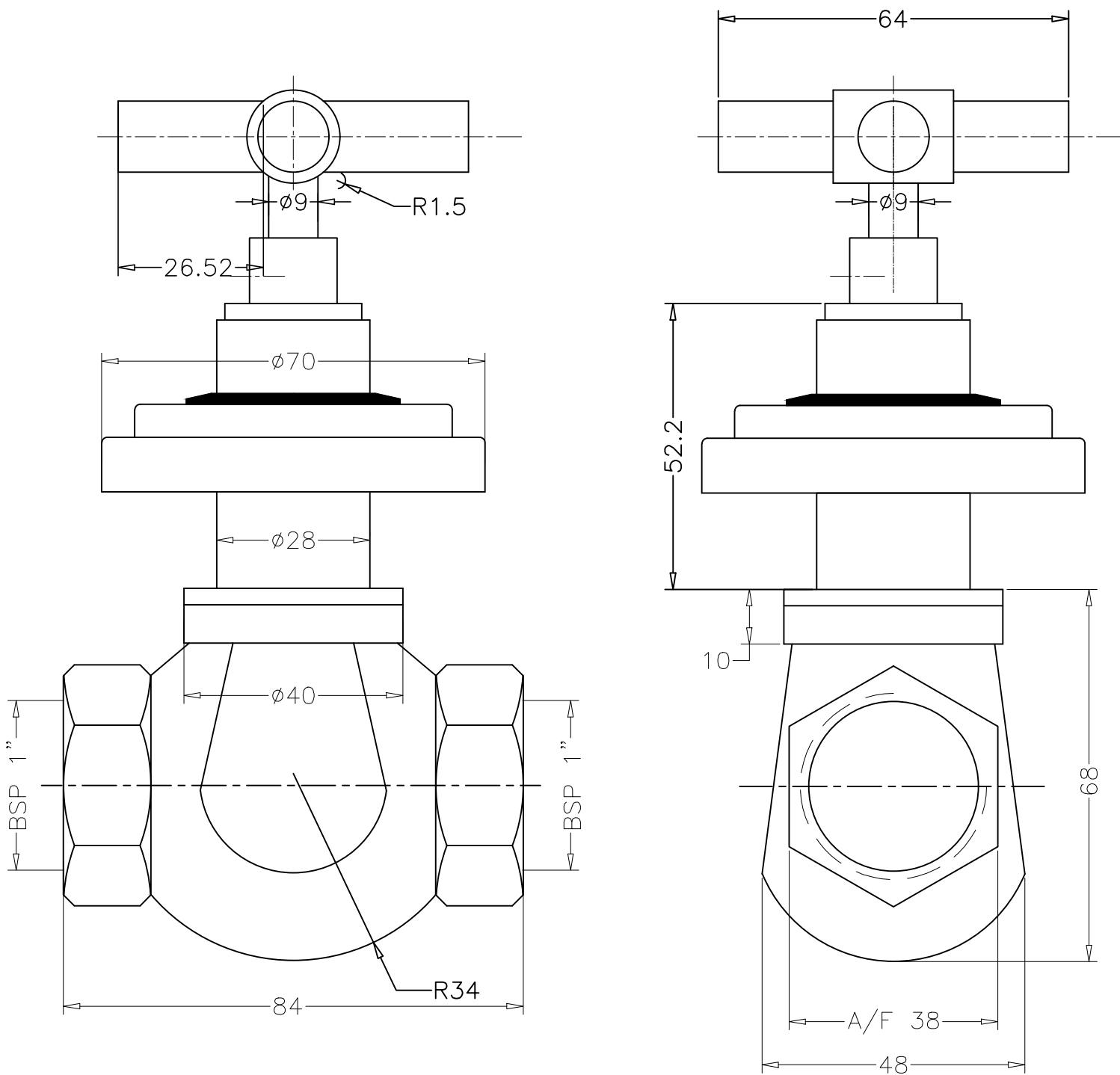
ADDONS-F850018 FLUSH COCK 25MM AXXIS HANDLE HALF TURN
